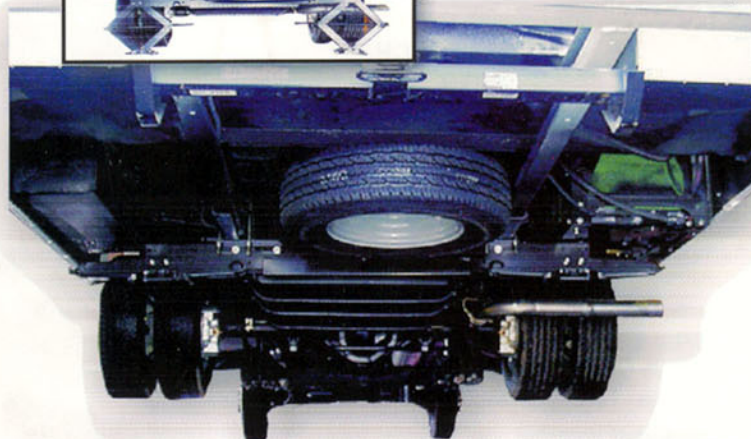
Rear jack system extended & retracted positions...
