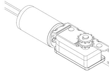
21900002 MOTOR & GEARBOX 68ZY SPROCKET UP HIGH TORQUE
