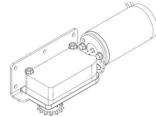
21900003 MOTOR & GEARBOX 68ZY SPROCKET DOWN HIGH TORQUE
