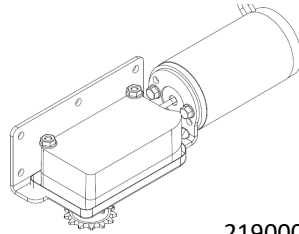
21900001 MOTOR & GEARBOX 64ZY SPROCKET DOWN
