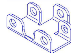
P854014 BRACKET, CHAIN / CABLE CONNECTOR
