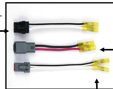
21700111 Service plug male 6" control end *Plugs into Control Box
